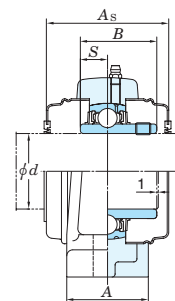
Pressed steel covers
