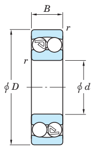
Cylindrical bore
