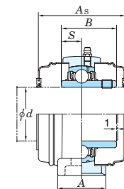
Pressed stainless steel covers
